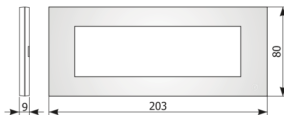
Ukrasni okvir 7M Decorative cover plate 7M
