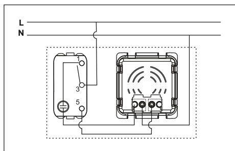
Kombo LED - Naizmjenična sklopka sa tinjalicom + LED u istoj montažnoj kutiji Kombo LED - Two-way switch with diffuser + LED in the same mounting box
