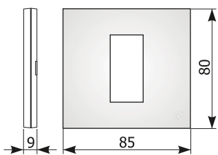
Ukrasni okvir 1M Decorative cover plate 1M
