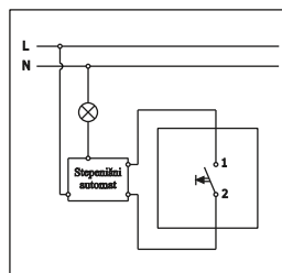
Taster svetla Light push-button
