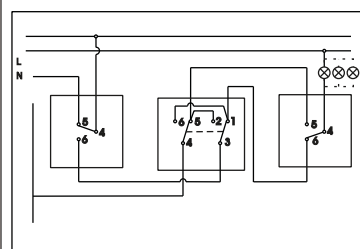
Unakrsna sklopka Intermediate switch
