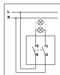
Dvopolna sklopka Double-pole switch
