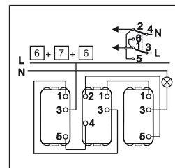
Kombo - Unakrsna sklopka Kombo - Intermediate switch - wiring
