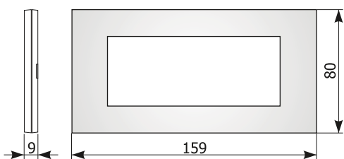
Ukrasni okvir 5M Decorative cover plate 5M
