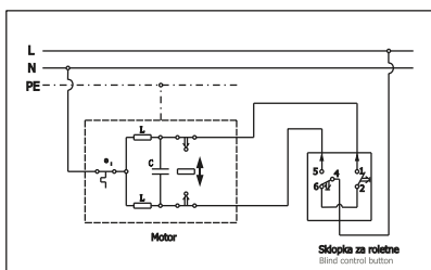
Taster za roletne i motor Wiring of blind control button and motor
