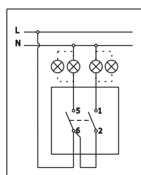
Dvopolna sklopka Double-pole switch
