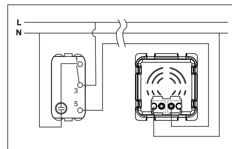
Kombo LED - Naizmjenična sklopka sa tinjalicom + LED u različitim montažnim kutijama Kombo LED - Two-way switch with diffuser + LED in the different mounting boxes
