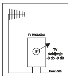
TV priključnica 1M prolazna TV aerial socket 1M feed through
