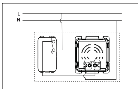
Kombo LED - Jednopolna sklopka + LED u istoj montažnoj kutiji Kombo LED - Single pole switch + LED in the same mounting box
