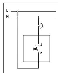
Taster zvona Bell push-button
