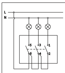
Tropolna sklopka Three-pole switch
