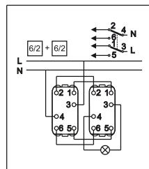
Kombo - Dvopolna naizmjenična sklopka Kombo - Two-way double-pole switch - wiring
