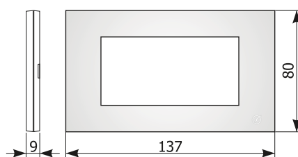
Ukrasni okvir 4M Decorative cover plate 4M
