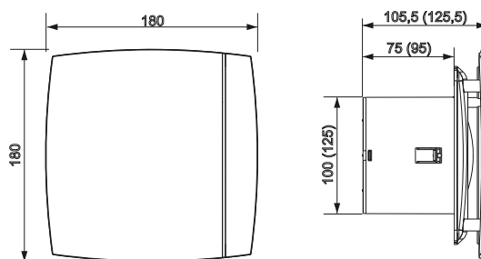
Ventilator za kupatilo-Fluent Panel 100 Bathroom fan-Fluent Panel 100
