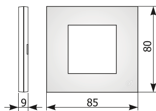
Ukrasni okvir 2M Decorative cover plate 2M
